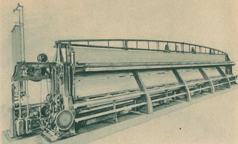
Automat-Schiffchenstickmaschine, Modell 18; 15 Yards.
